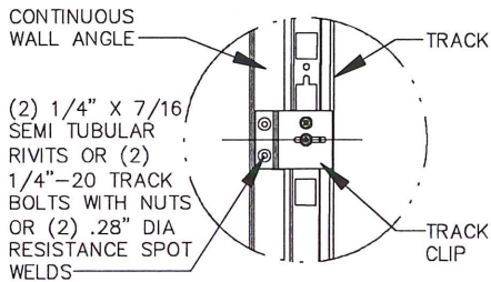
DETAIL F
